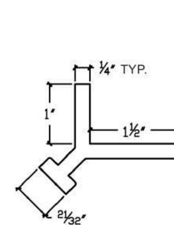
1" Embedment Angle
