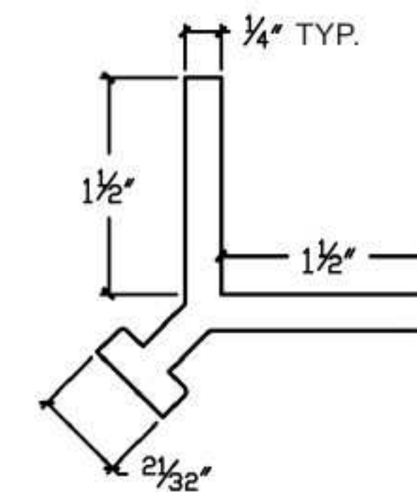
1 1/2" Embedment Angle
