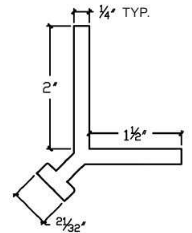
2" Embedment Angle
